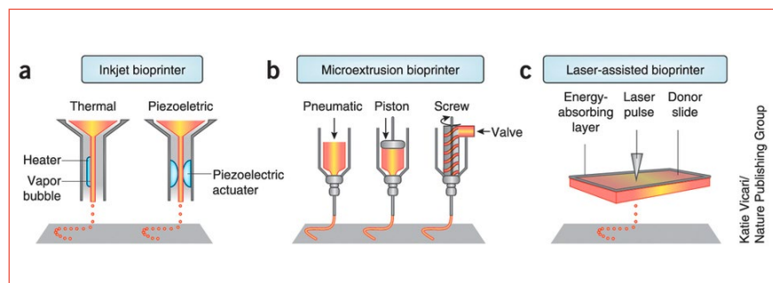
FIGURE 2 The three main bioprinting techniques: (a) Inkjet bioprinting; (b) Microextrusion bioprinting; (c) Laser-assisted bioprinting (LAB)
